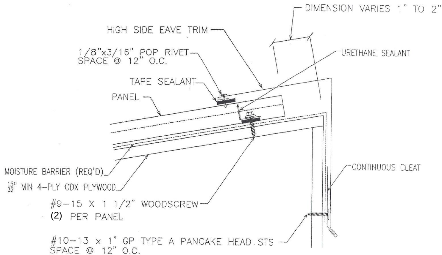
7 SECTION THRU HIGH EAVE
