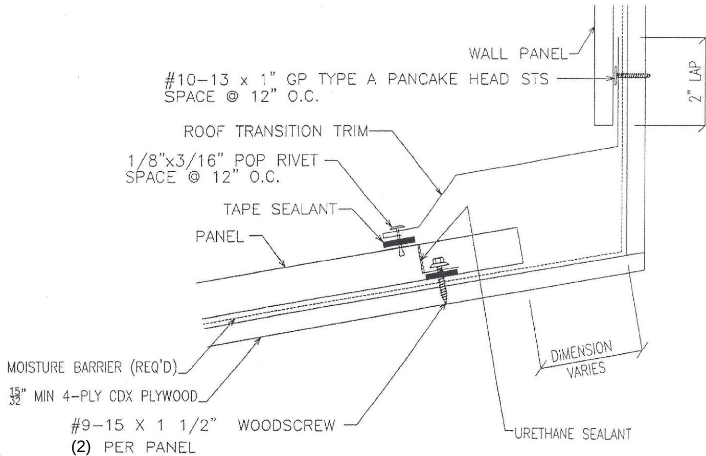
8 SECTION THRU HIGH SIDE TRANSITION
