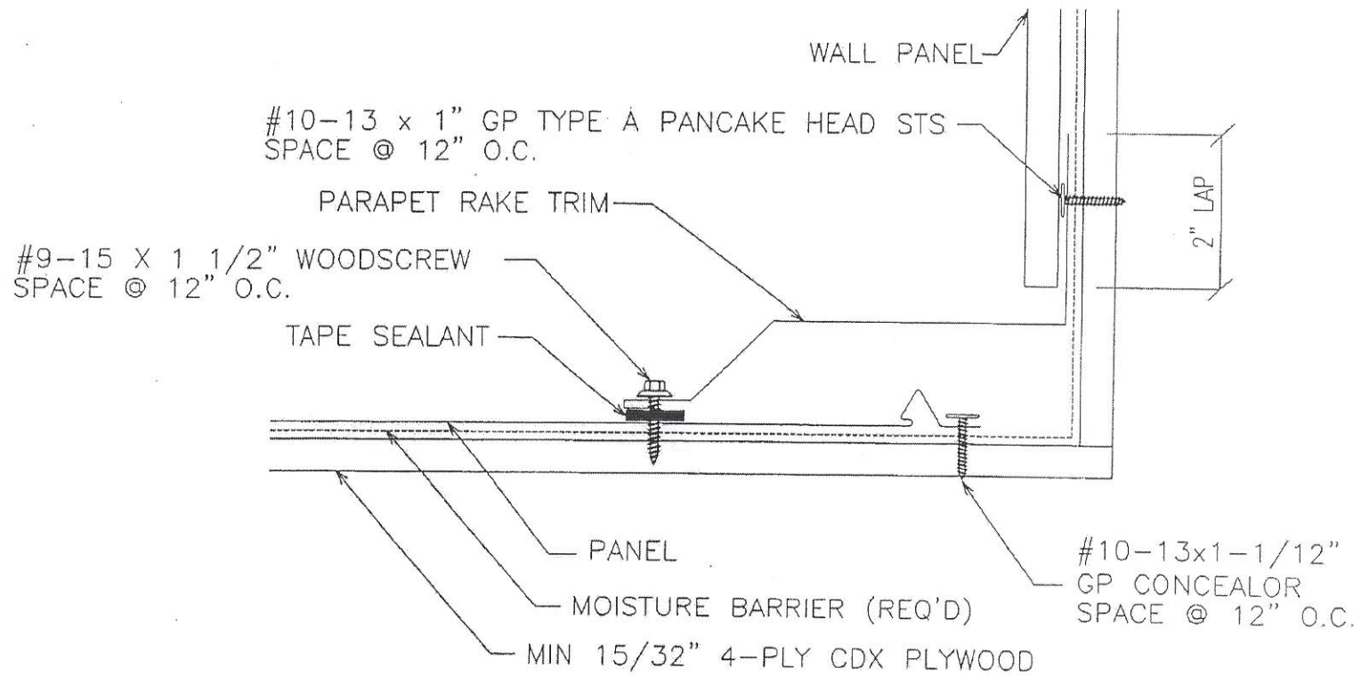
10 SECTION THRU RAKE PARAPET
