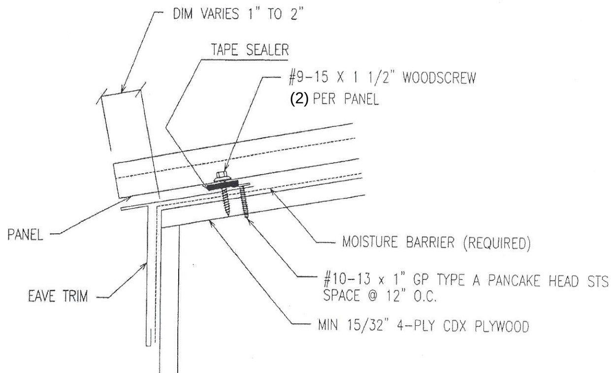
① SECTION THRU EAVE
