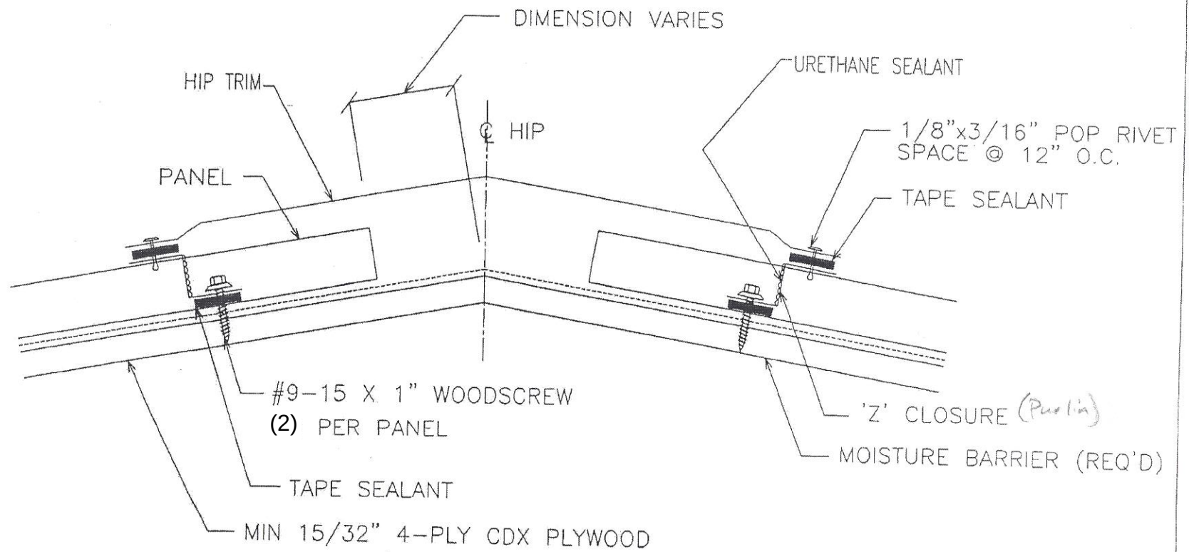
9 SECTION THRU HIP
