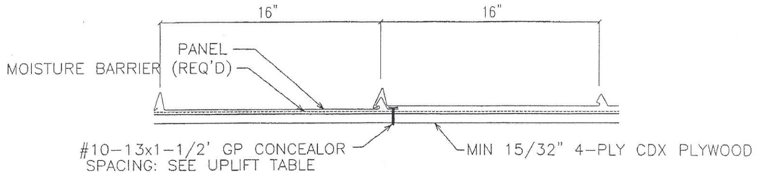
FASTENER LOCATION AT PANEL INTERIOR
