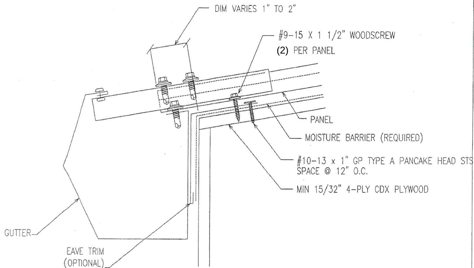
2 SECTION THRU EAVE W/ GUTTER
