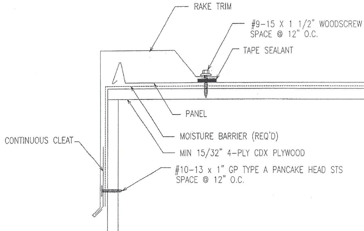
5 SECTION THRU RAKE
