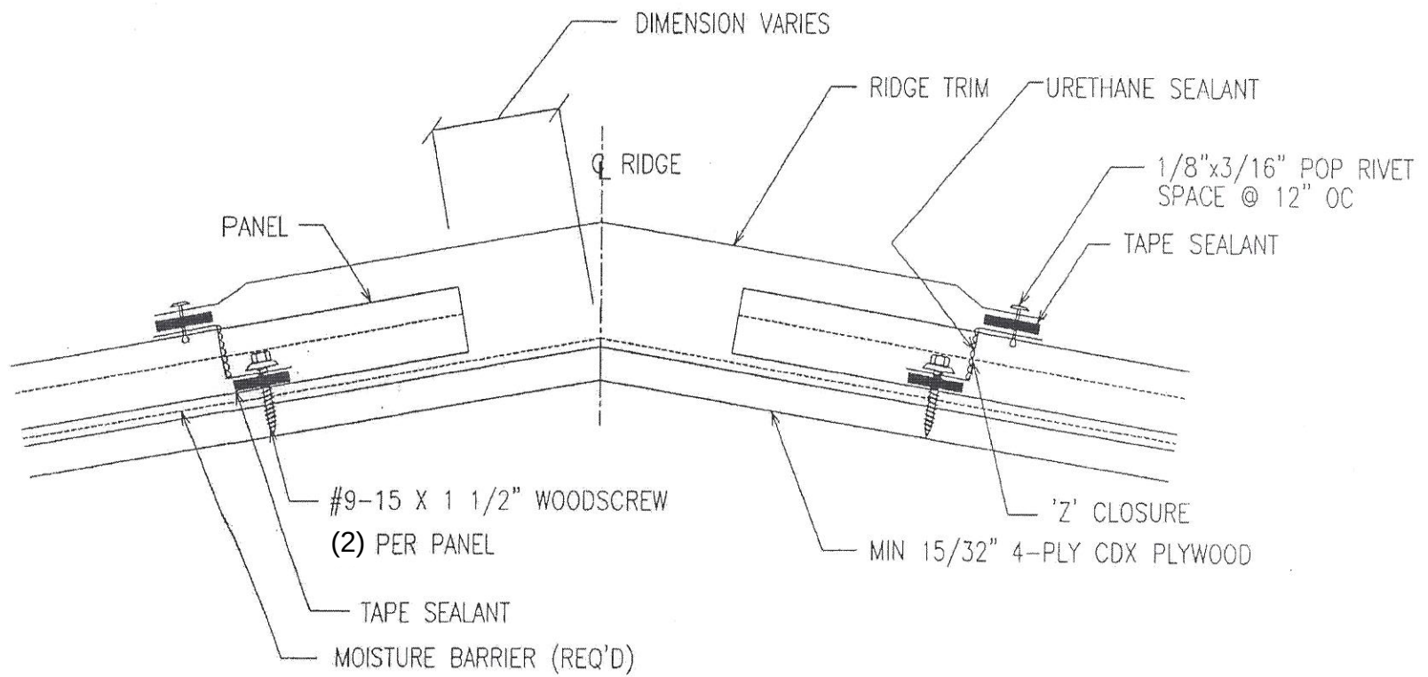
4 SECTION THRU RIDGE
